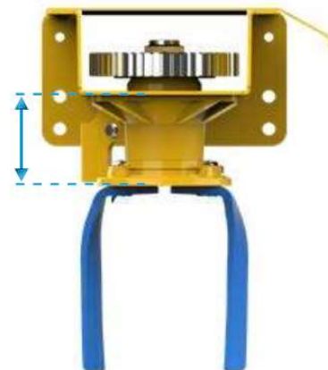
TWIN FORCE MAX Clearance 165 mm
