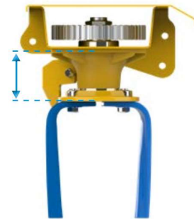
TWIN FORCE TEK Clearance 130 mm
