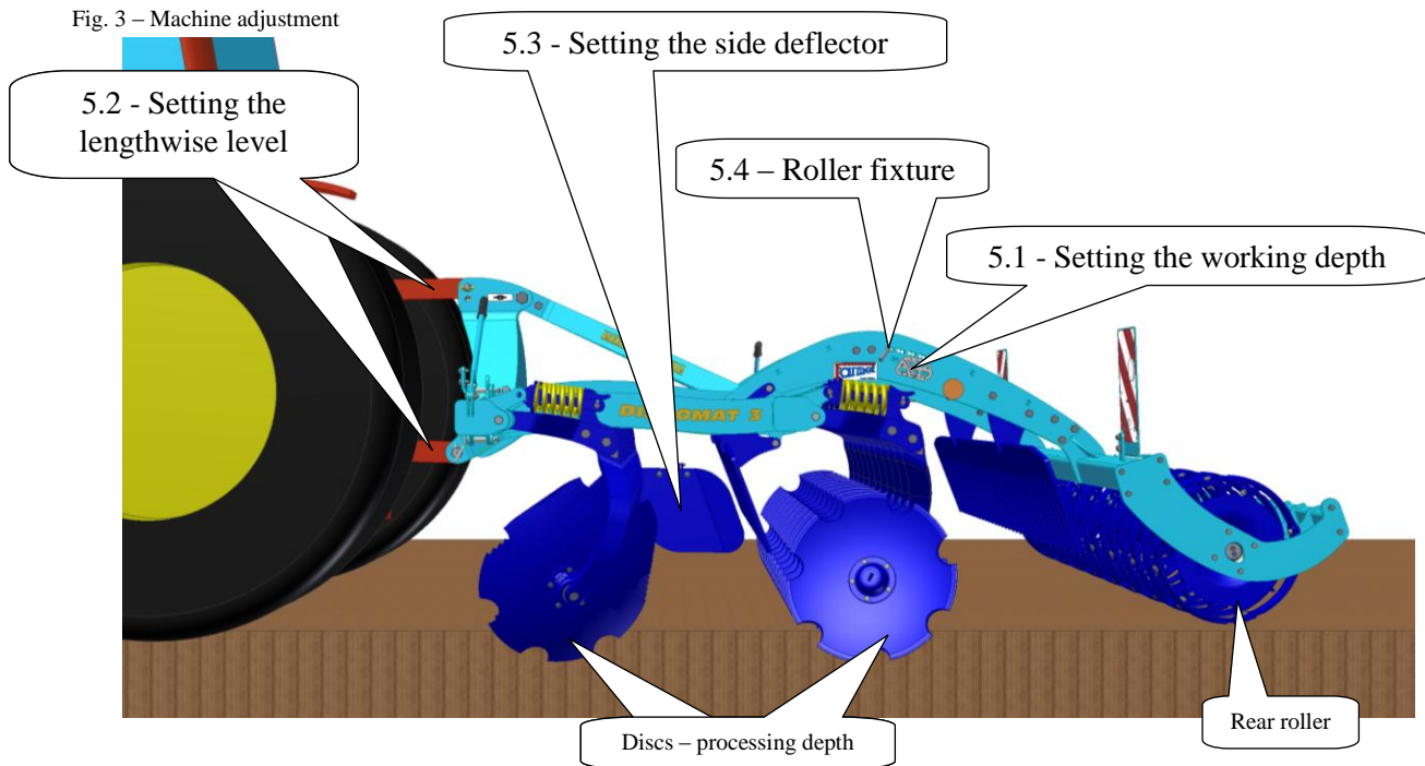
Fig. 3 – Machine adjustment
