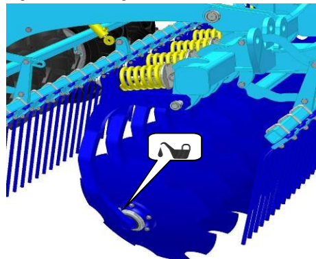
Fig. 5 - Disc bearings
