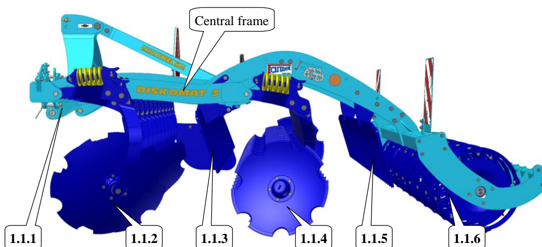
Fig. 2 – Work Parts of the Machine
