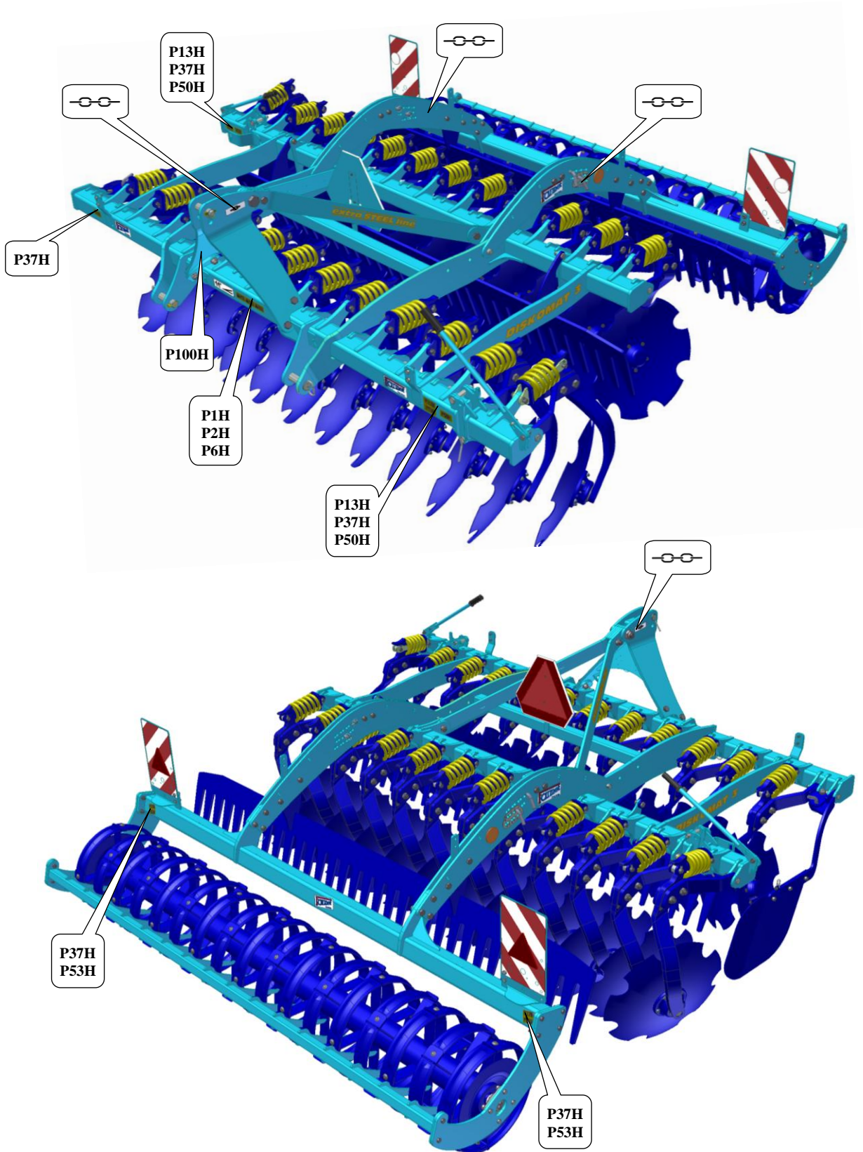
Fig. 1 - Location of safety labels on the DISKOMAT machine
